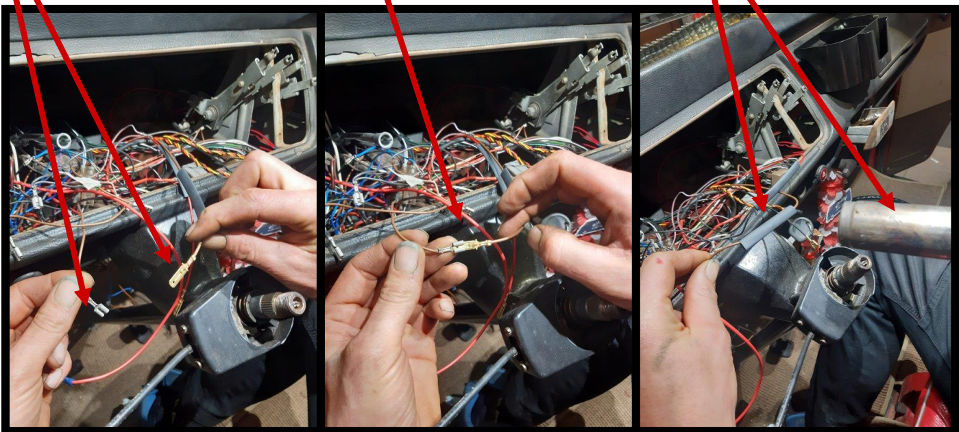
Classic Evo Gauge Connect the brown cable of the Classic Evo Gauge to the Brown/Black cable (this is the cable that goes from the float to the original gauge) of the car
