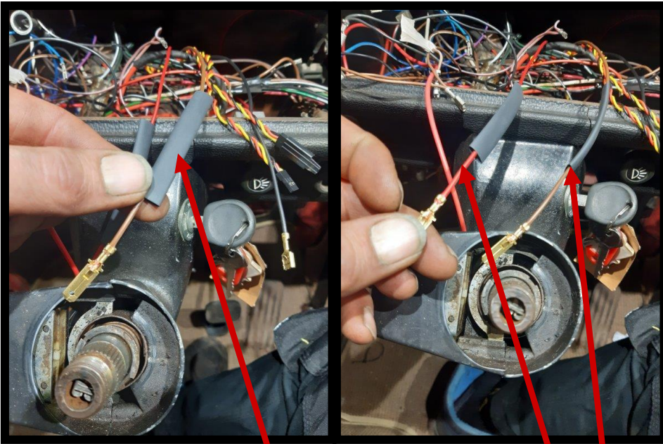
Classic Evo Gauge Slide the heat shrink tubing over both the Brown and Red cables of the Classic Evo Gauge
