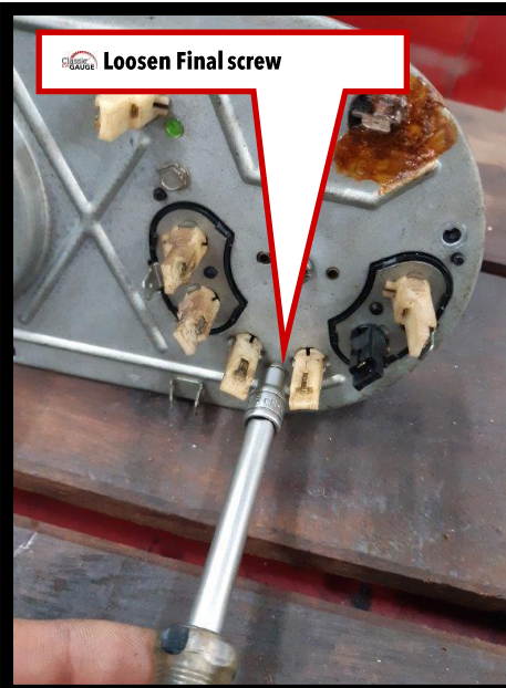
Disassemble plastic housing
